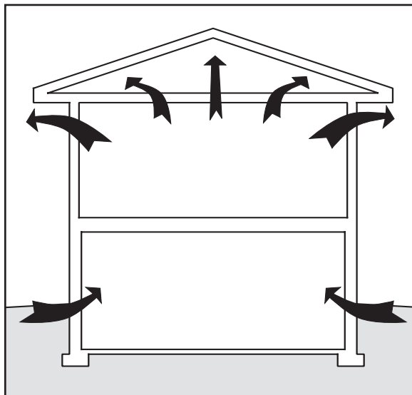
Figure 1 During the winter, warm air inside the house will cause the house to act like a big chimney, drawing air in at the lower parts of the house and exhausting the warm and moistened air wherever there is an opening in the wall or ceiling. This is called the "stack effect."
