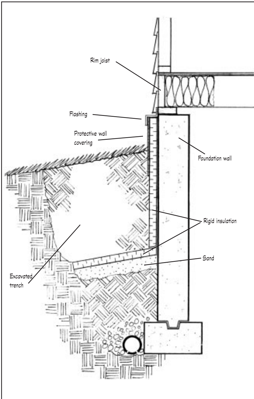
Figure 3 Basic parts of the foundation wall and the exterior insulation "apron" method.
